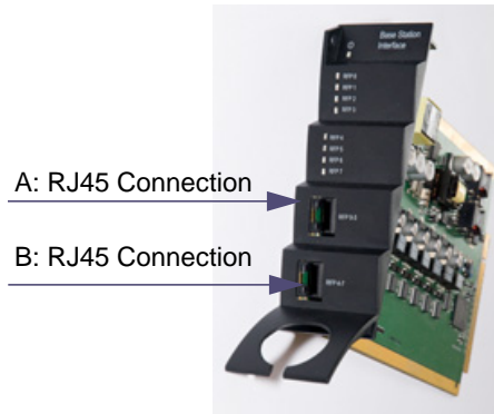
Figure 2 RJ45 Connections for Base Stations
